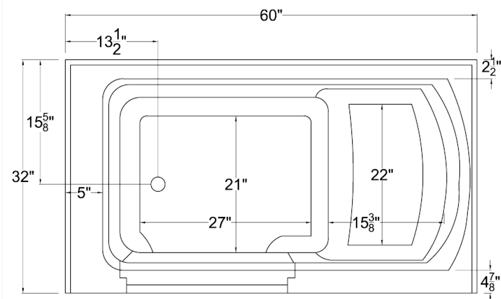
TOP VIEW
