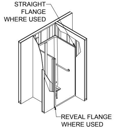
TYPICAL FRAMING
